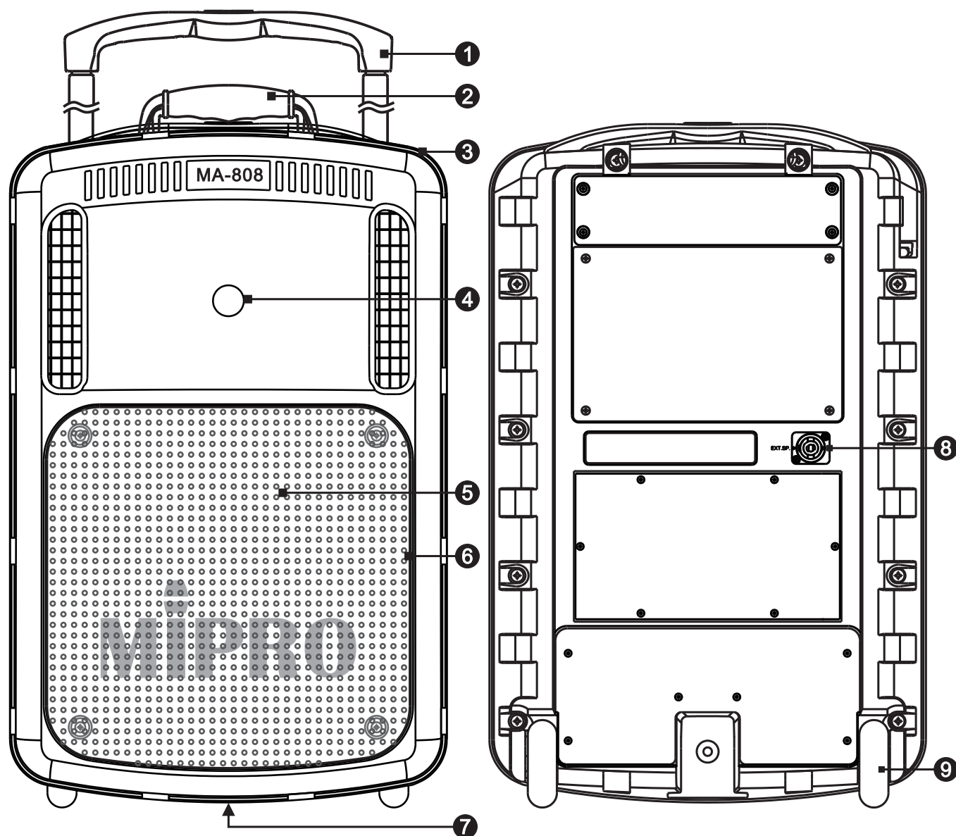
Front Panel
