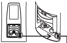
Switch the latch left to block the power switch Fig. 25
